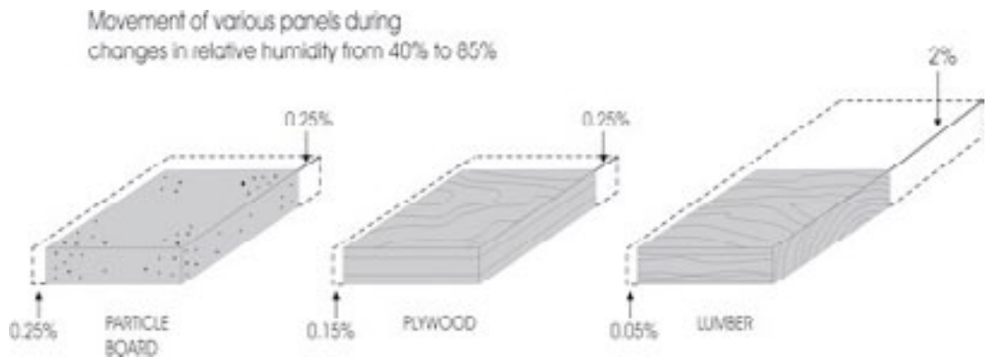
Figure 22: In-plane movement of various panels
