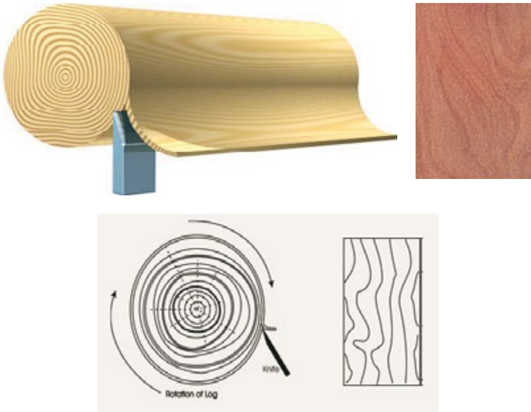
Figure 2: Rotary peeling of veneers
