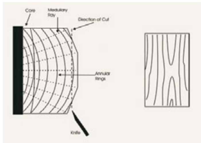
Figure 5: Crown cut or flat slicing of veneer
