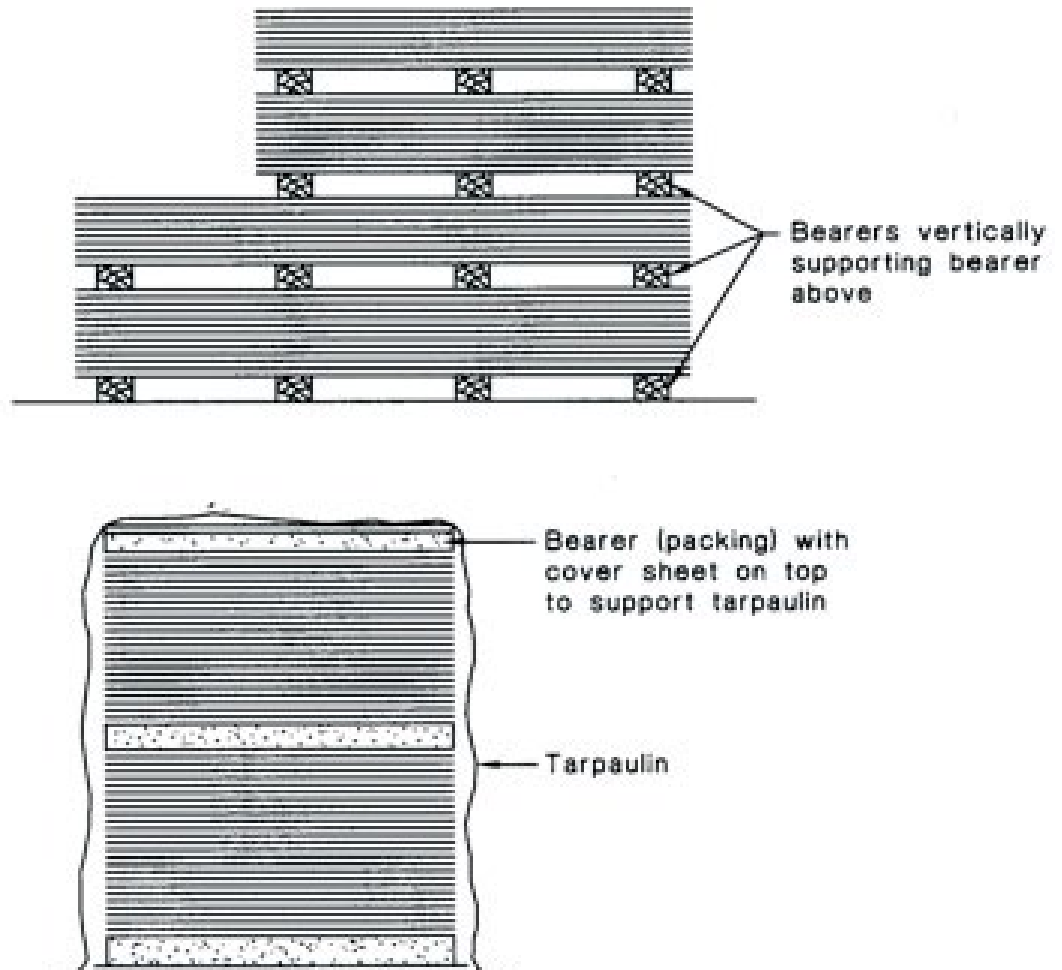
Figure 25: Recommended storage and handling of decorative veneered panels (top) Correct storage method (bottom) Temporary cover Source: AS/NZS 1859.3: 2005
