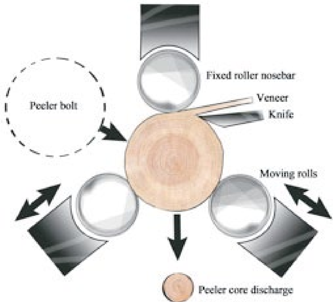
Figure 3: Principles of peeling with a spindleless lathe
