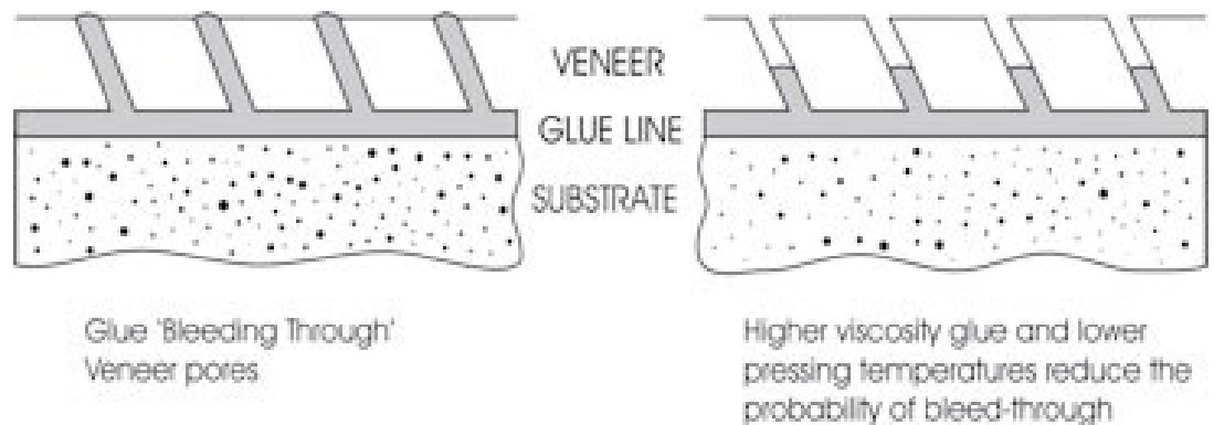
Figure 41: Glue bleed-through
