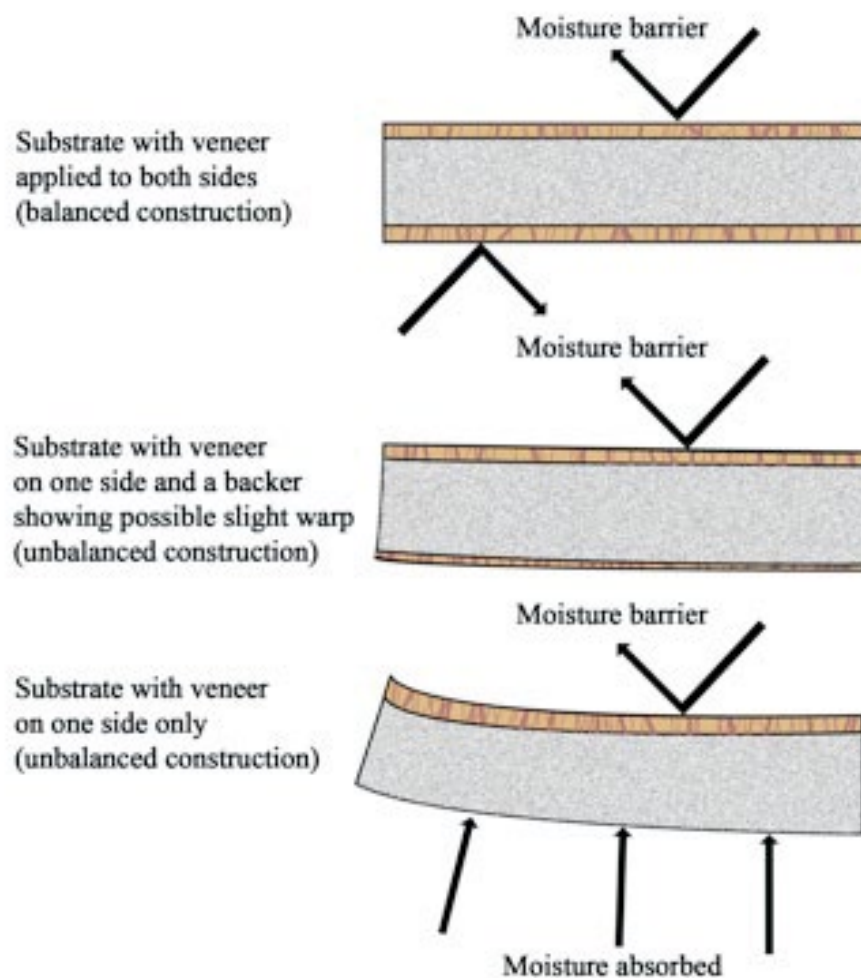
Figure 23: Balanced and unbalanced construction of veneered panel
