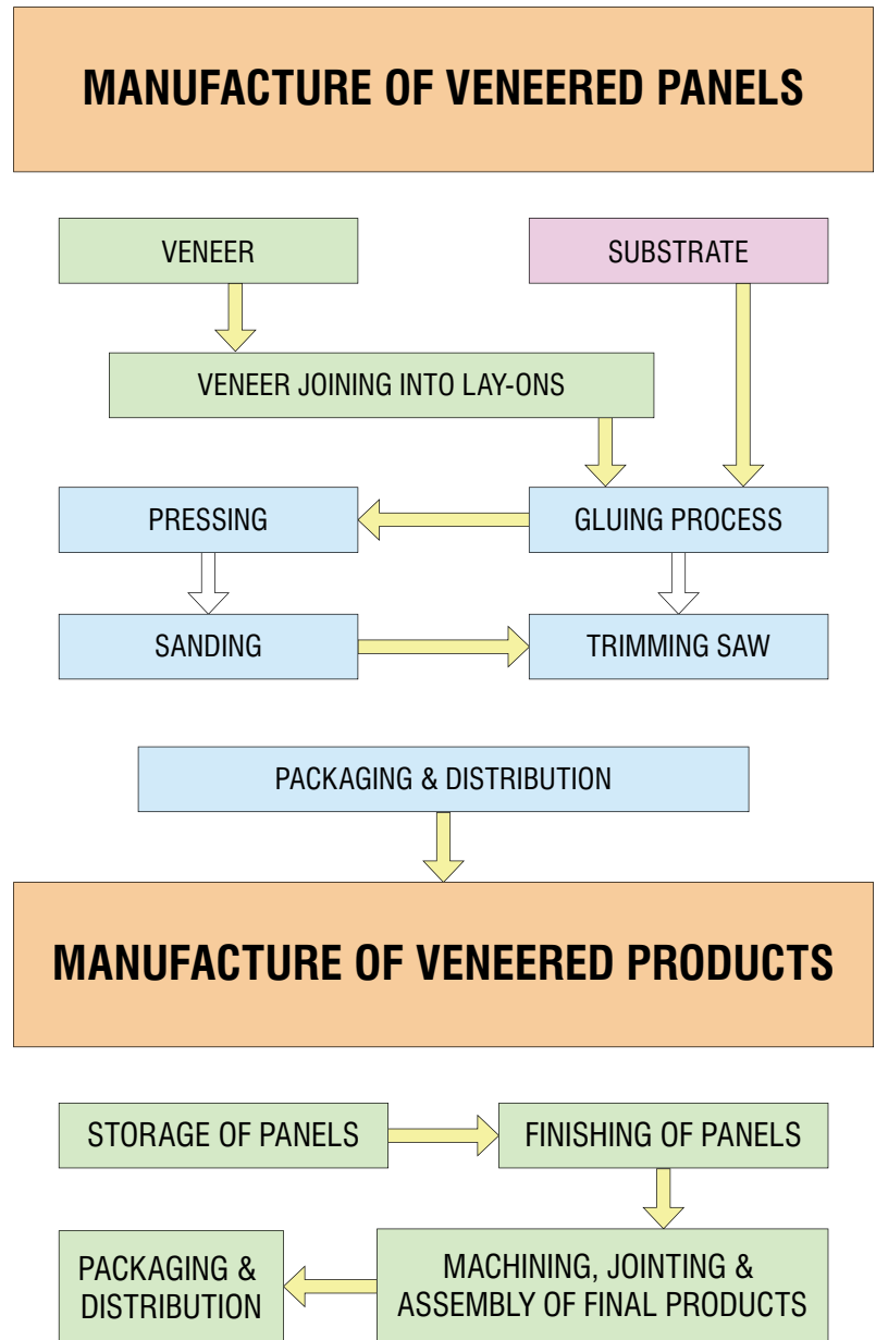
Figure 24: Manufacturing stages in the production of veneered products
