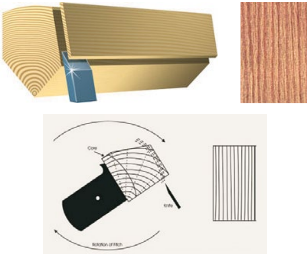
Figure 8: Rift cut slicing of veneer
