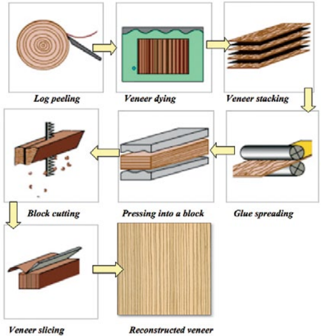
Figure 9: Production of reconstructed veneer
