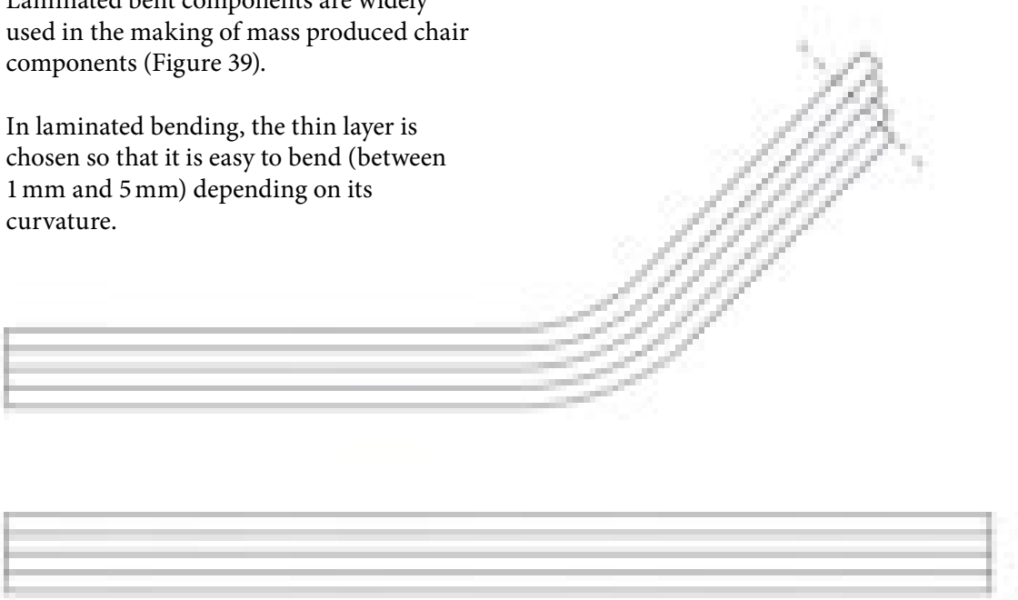
Figure 38: Laminated bent component
