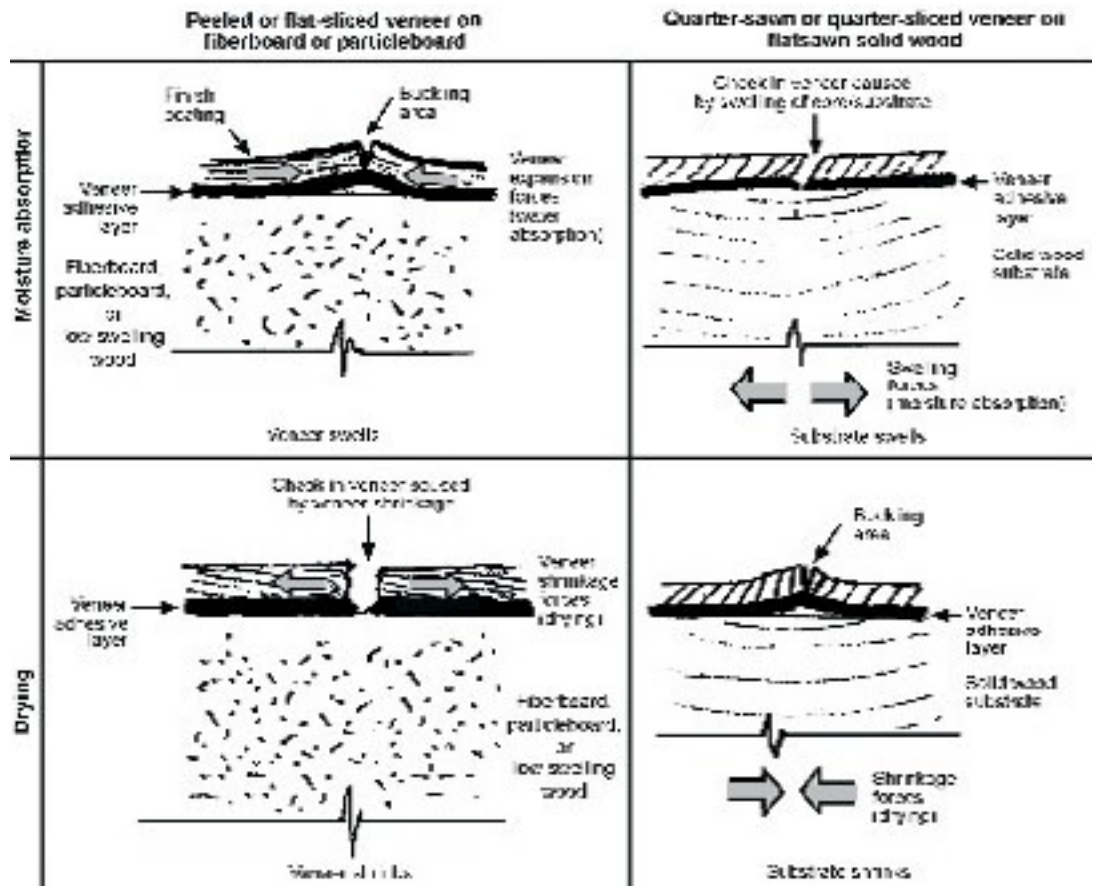
Figure 44: The formation of checks caused by differences in swelling and shrinkage characteristics.
