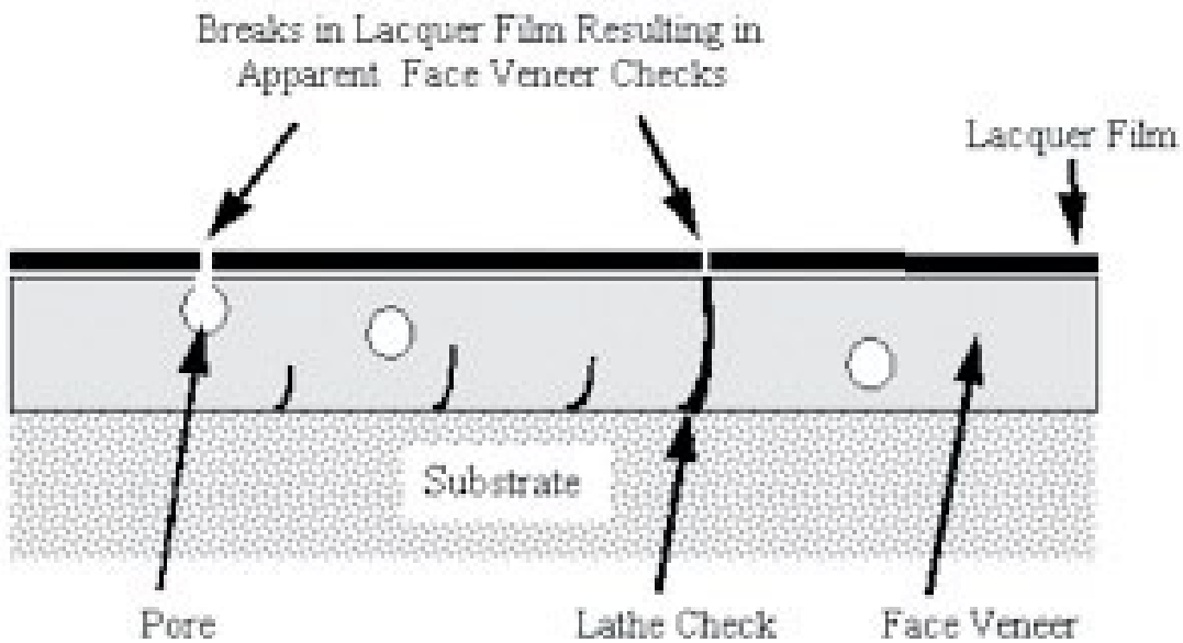
Figure 43: Veneer checks as the result of wood failure in the face veneer
