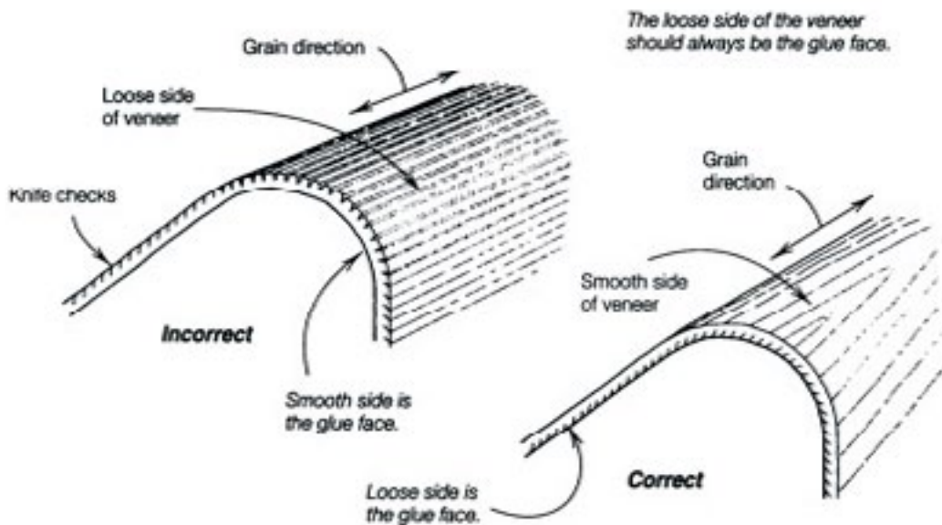
Figure 35: Loose and tight side of veneer
