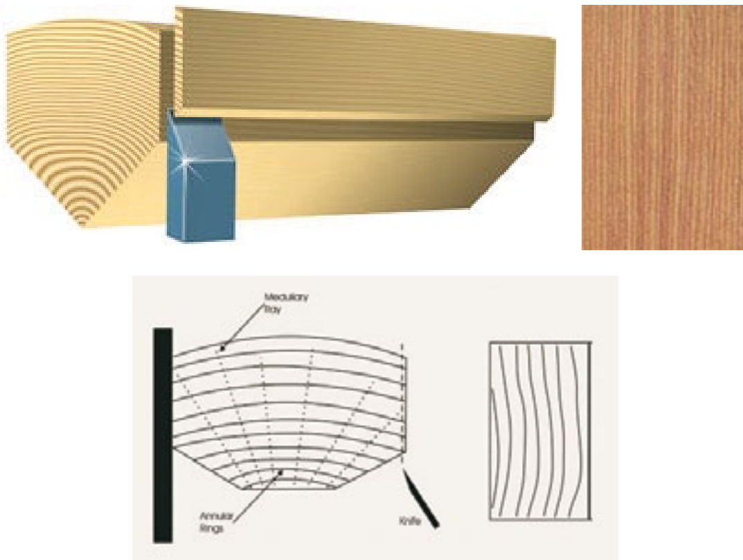
Figure 4: Quarter slicing of veneer
